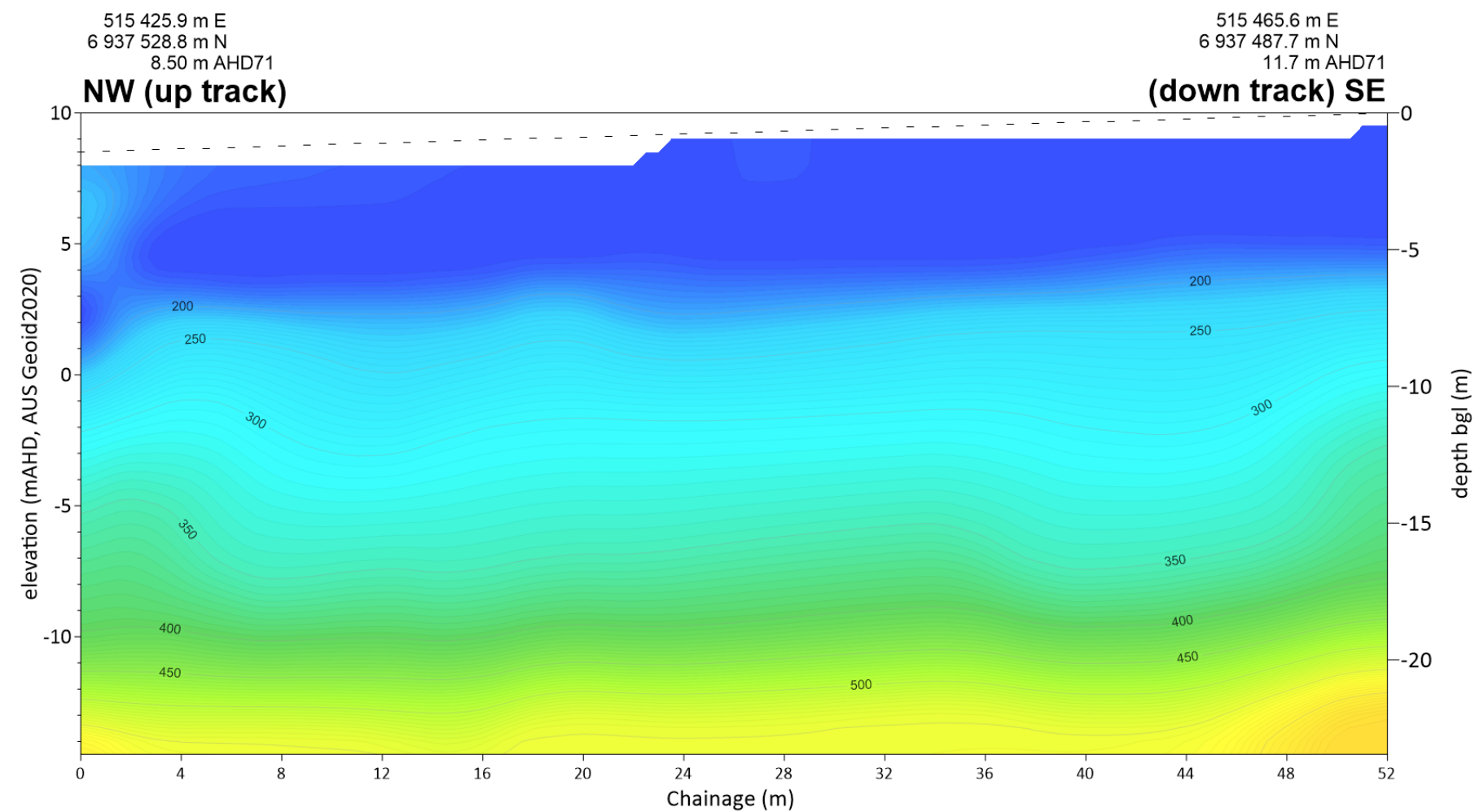
Seismic Line MASW AU-GP 162-1
